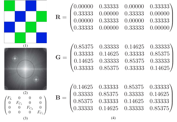
Fig. 4. The proposed Circ4 CFA pattern. (1) is the proposed 4 \times 4 circulant CFA pattern. (2)-(4) are its spectrum, frequency structure, and color values, respectively. The notations in (2) and (3) are the same as those in Fig. 1.
