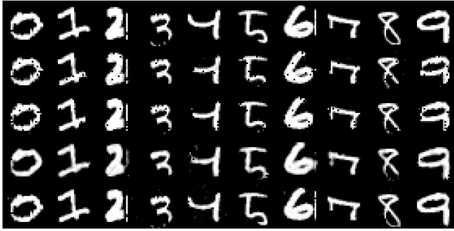
Fig. 6. Reconstructions using multi-layer autoencoders trained on the MNIST dataset. The top row is original images. The following rows are the results of autoencoders trained by Adam, AMSGrad, SGD, and sync-LPOM, respectively.
